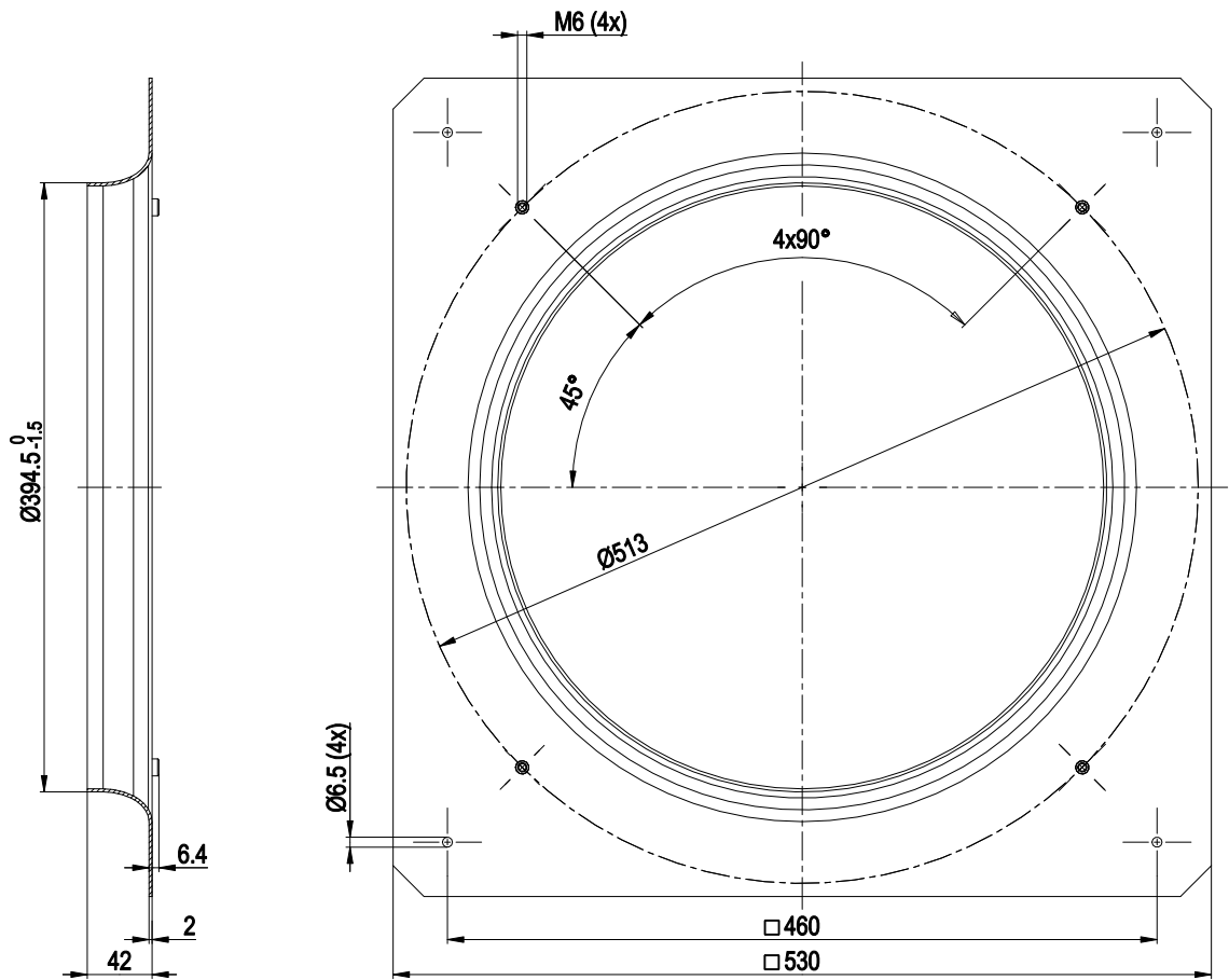
Inlet ring 40100-2-4013
