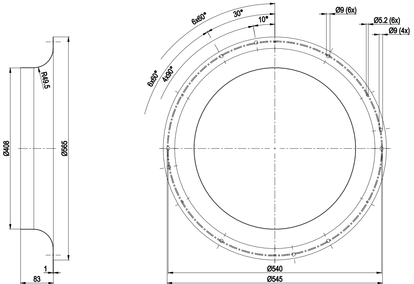
Inlet ring 54482-2-4013
