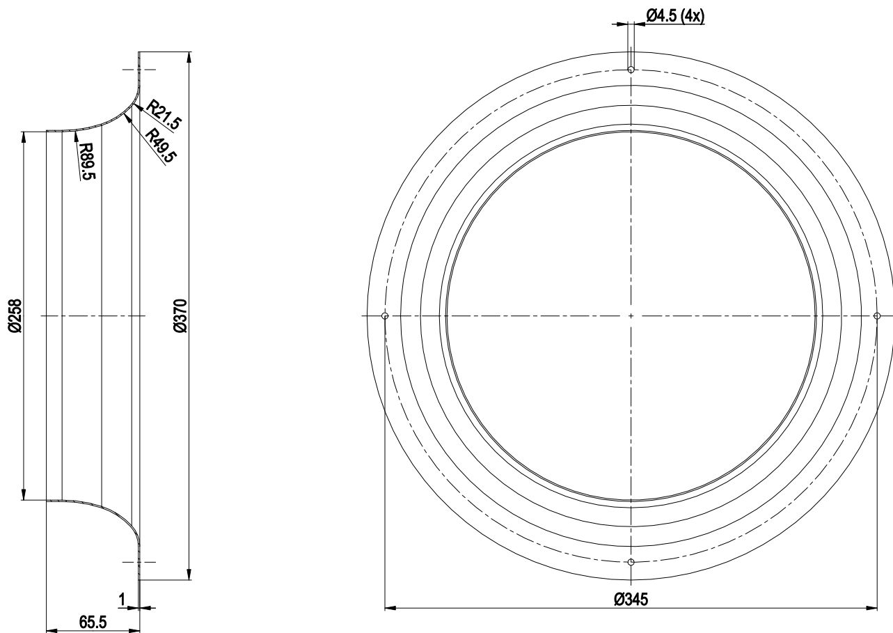
Inlet ring 54476-2-4013
