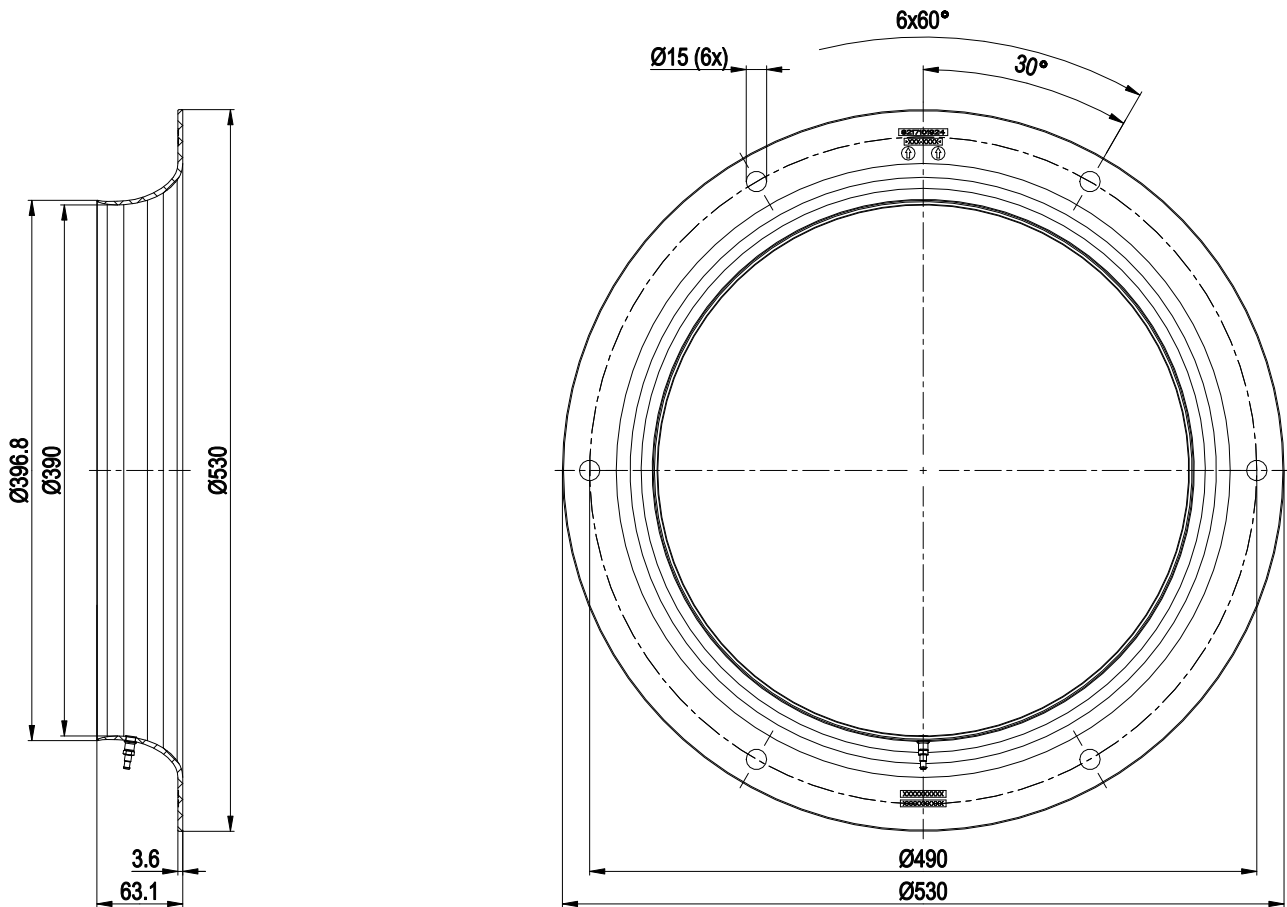
Inlet ring 8217102237 with pressure tap (k-factor: 381)
