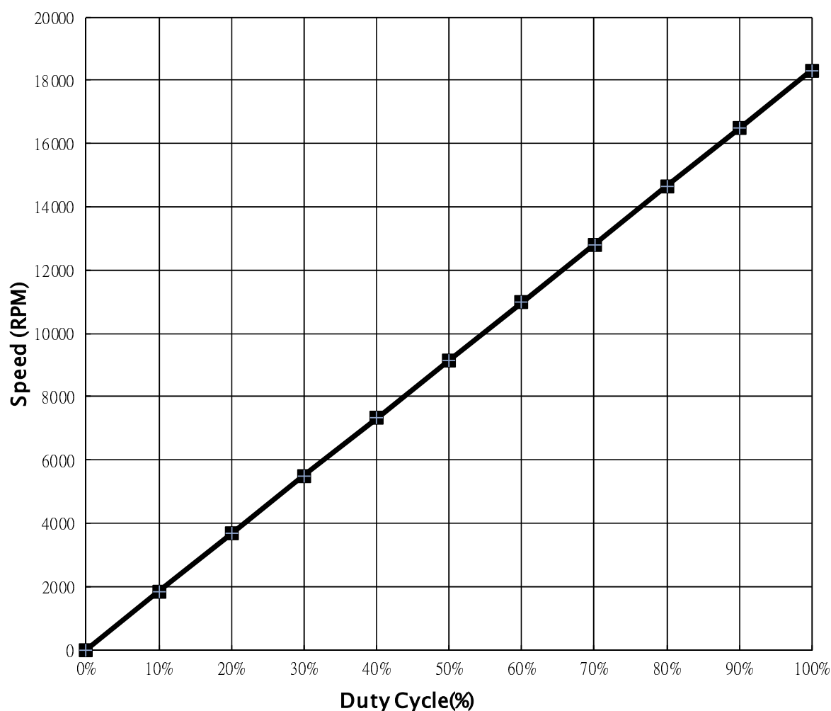
Duty Cycle v.s. Speed curve
