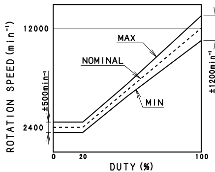
Detail of PWM curve(At 0~100%)
