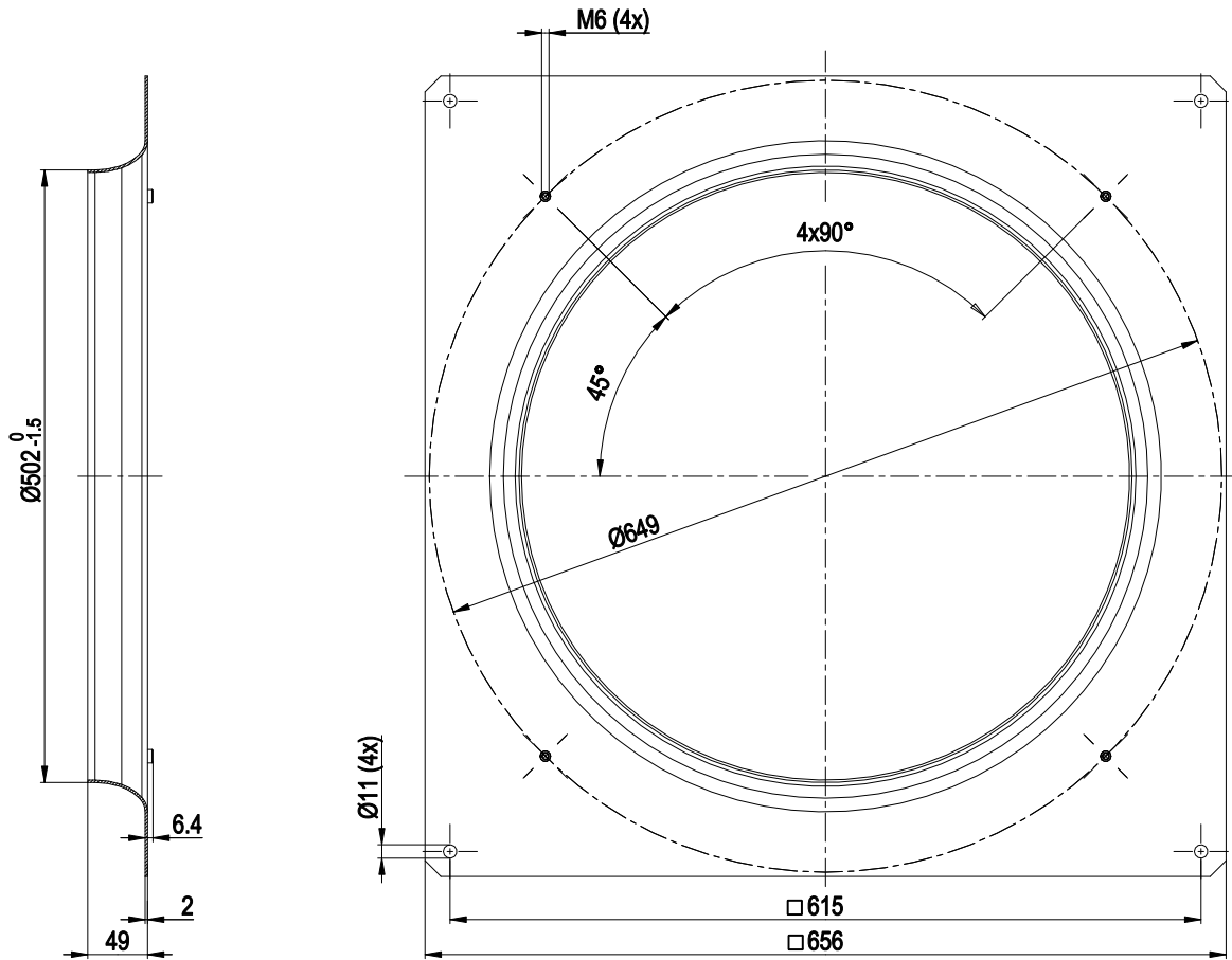
Inlet ring 50100-2-4013
