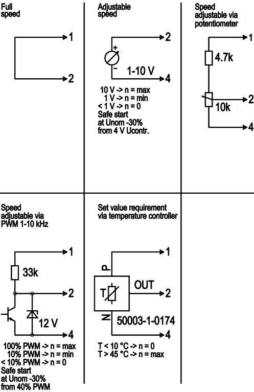
Customer circuit
