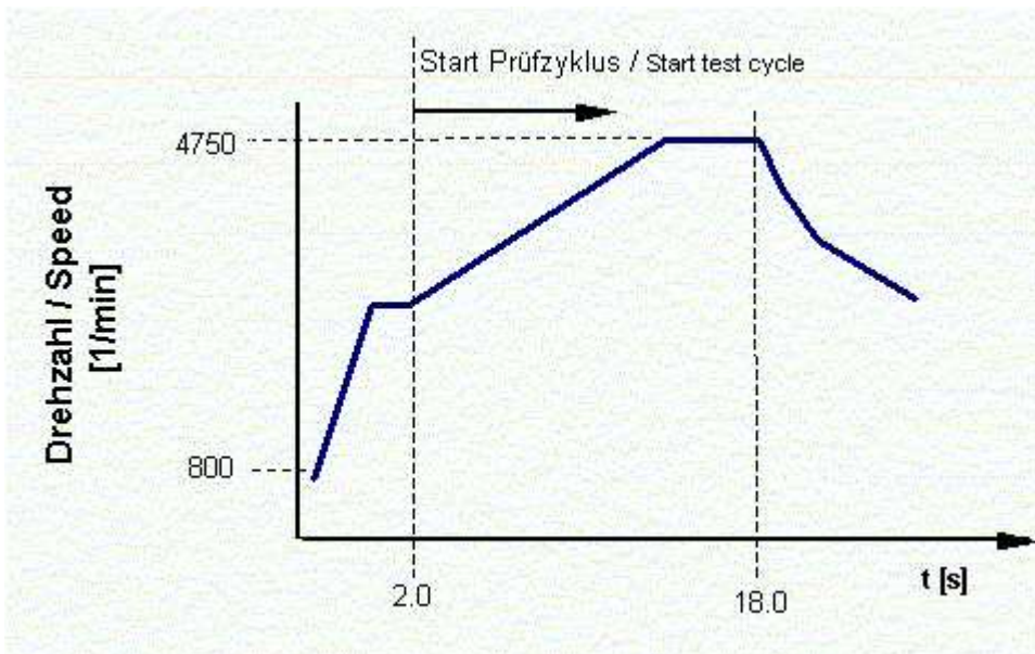
Speed graph after starting the test cycle
