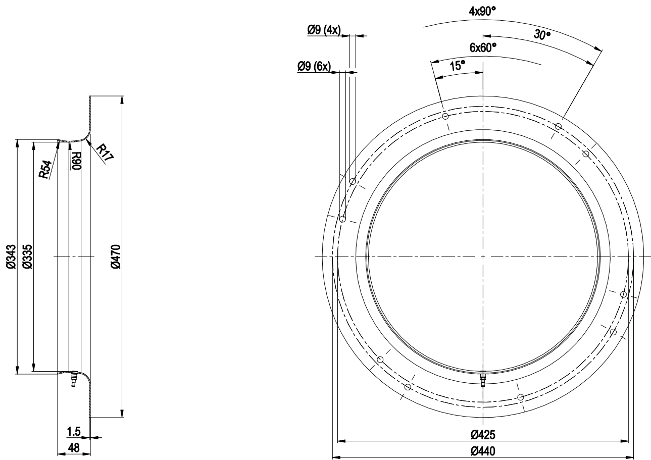
Inlet ring 45355-2-4013 with pressure tap (k-factor: 250)
