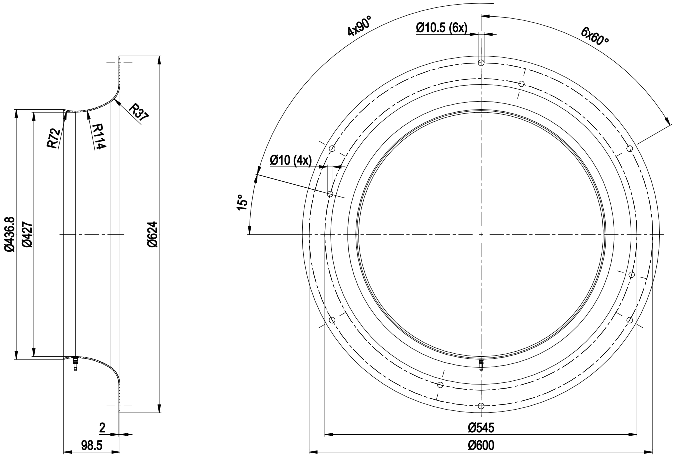
Inlet ring 64040-2-4013 with pressure tap (k-factor 438)
