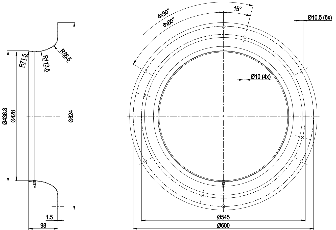
Inlet ring 64040-2-4013 with pressure tap (k-factor 438)
