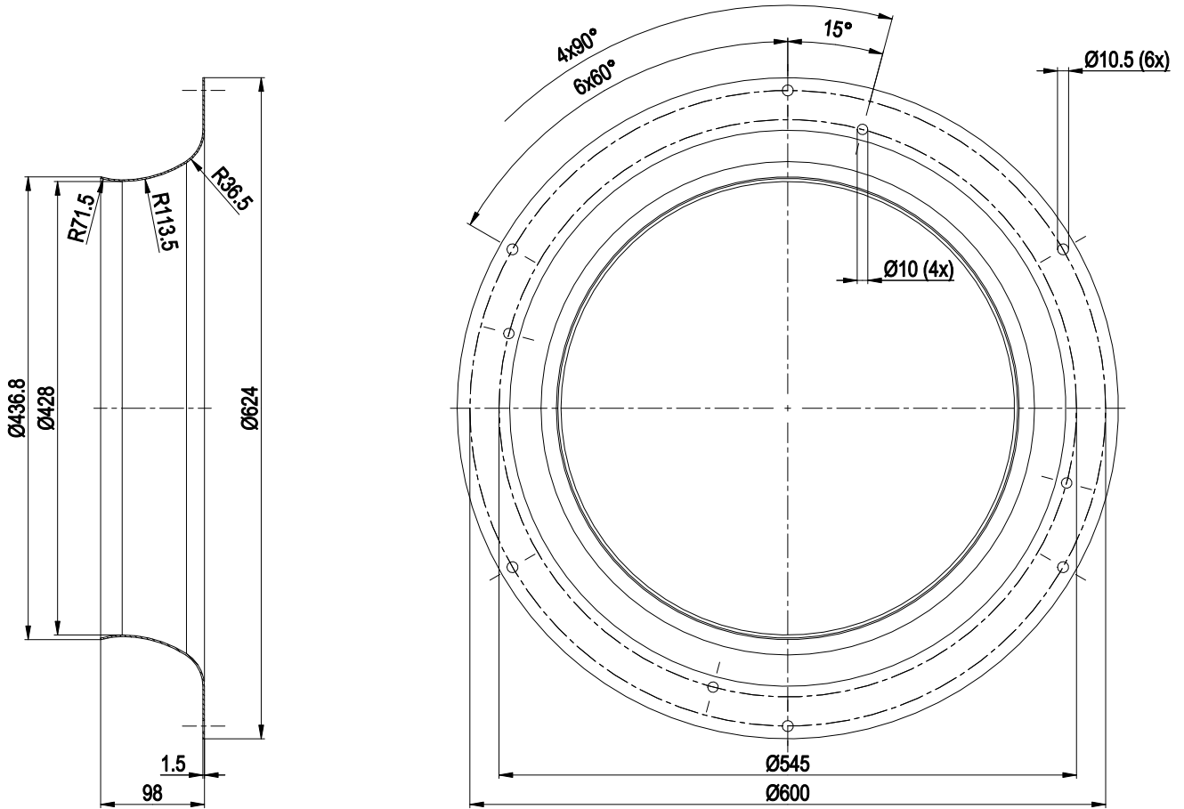
Inlet ring 63070-2-4013
