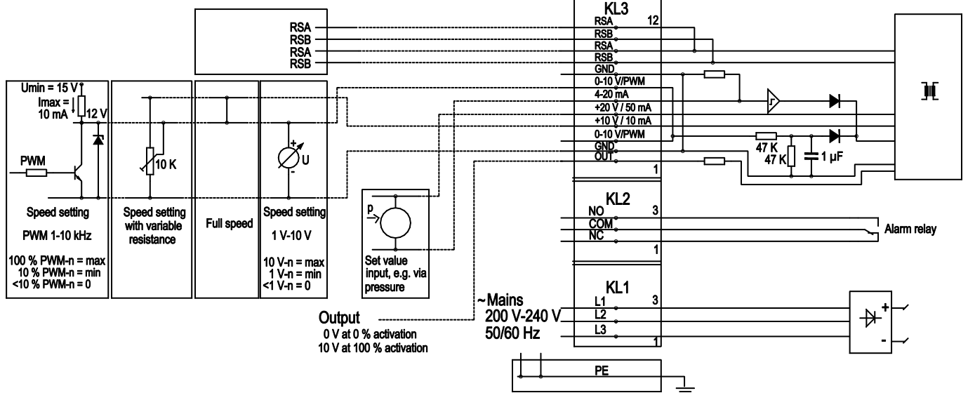
Customer circuit
