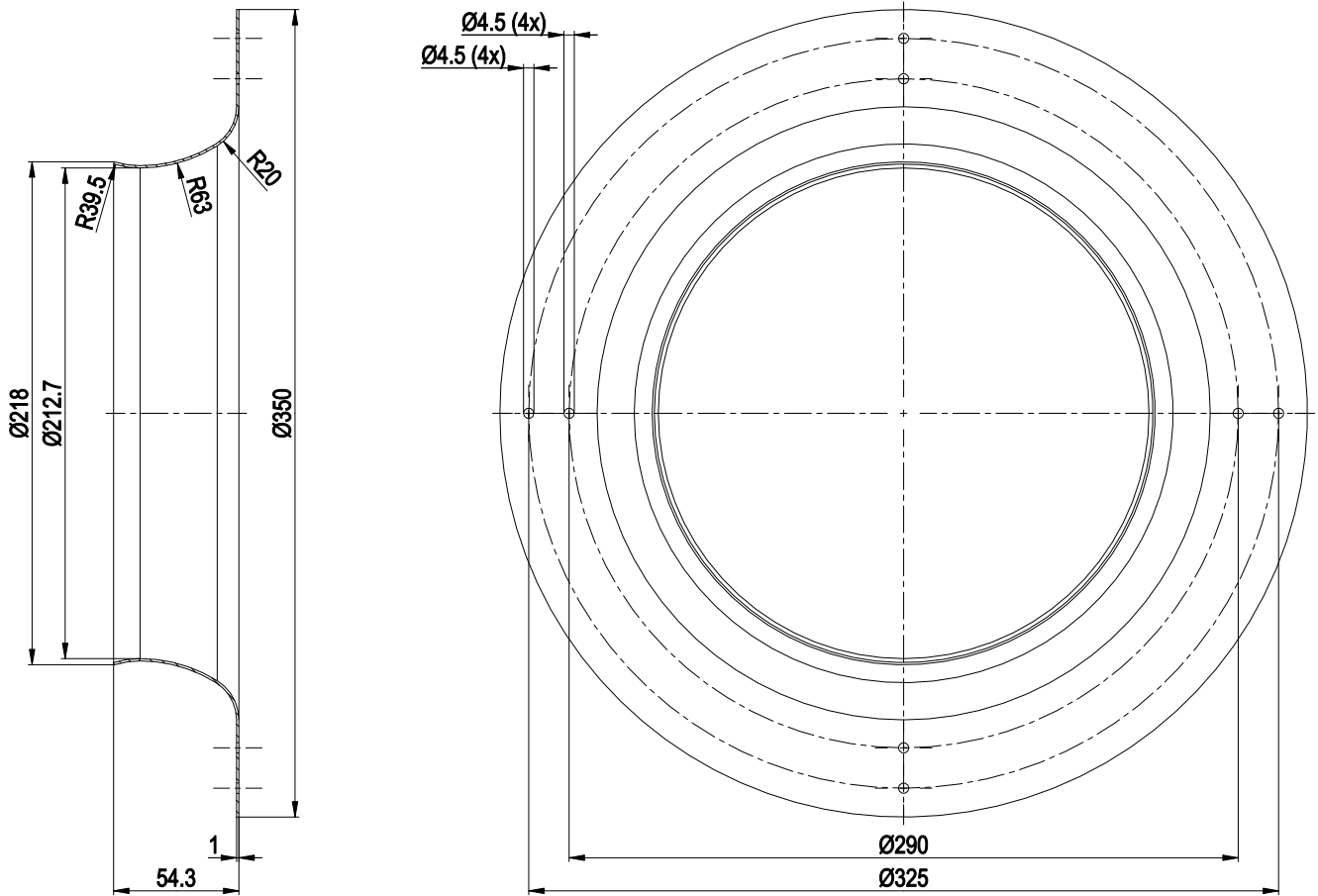
Inlet nozzle 31570-2-4013
