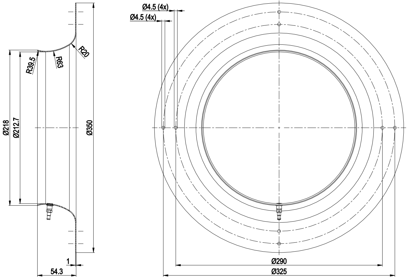
Inlet ring 31575-2-4013 with pressure tap (k-factor: 116)
