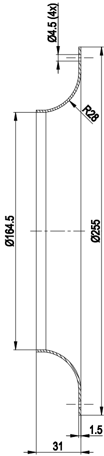
Inlet ring 96359-2-4013
