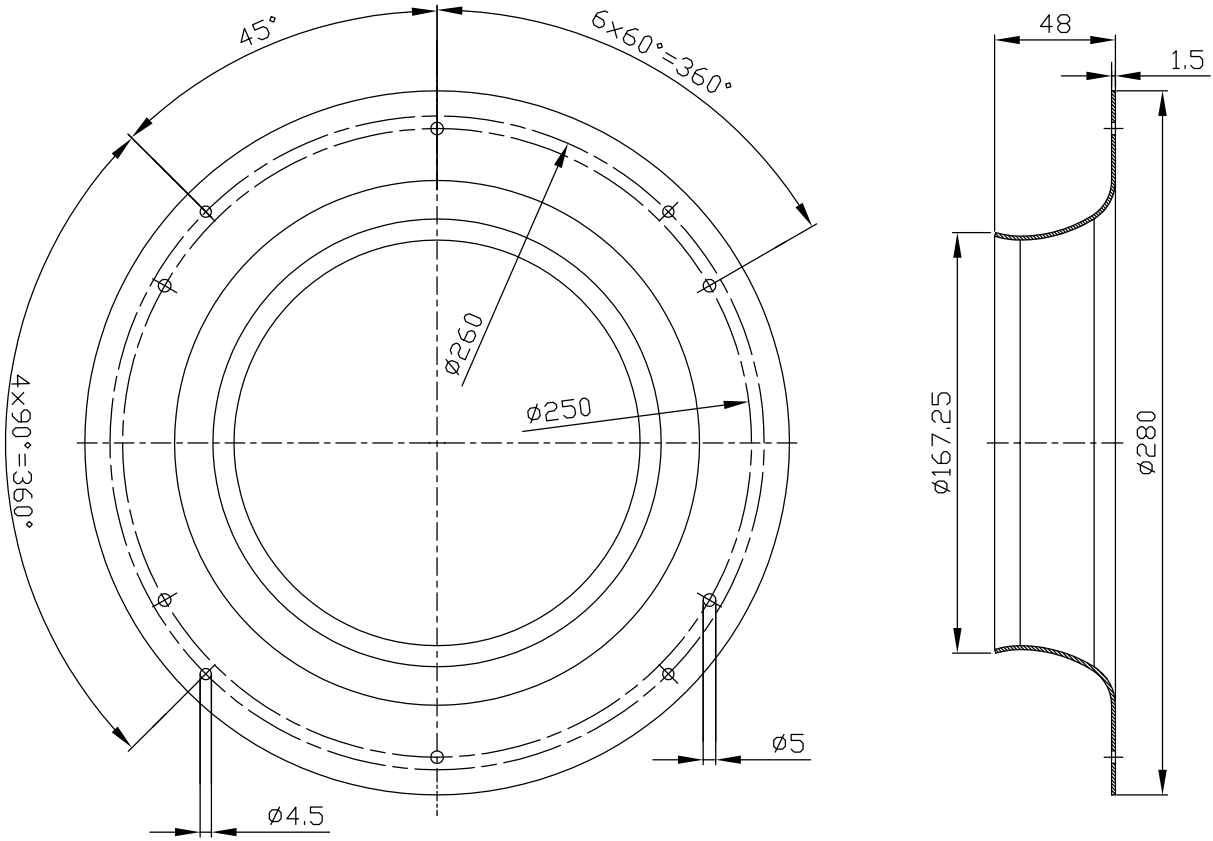
Inlet ring 96350-2-4013
