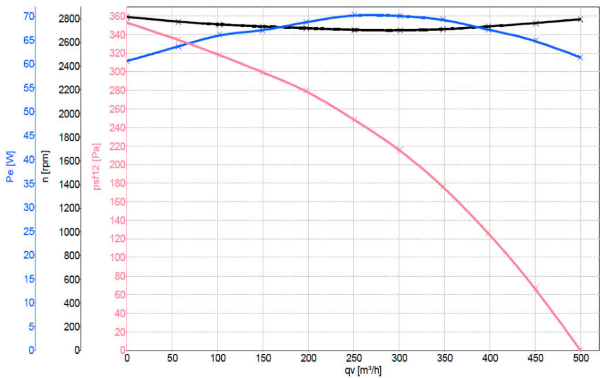
Charts: Air flow 50 Hz
