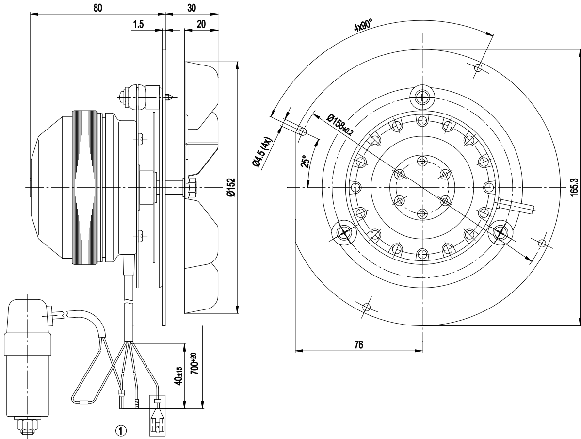
1 Connection line PFA AWG20; 1x core-end sleeve, 1x brass lead tip and 1x receptacle for tabs 6.3 x 0.8 with housing, crimped
