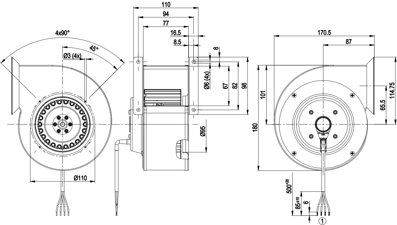
1 Cable PVC 4G 0.5 mm 2 , 4x crimped splices
