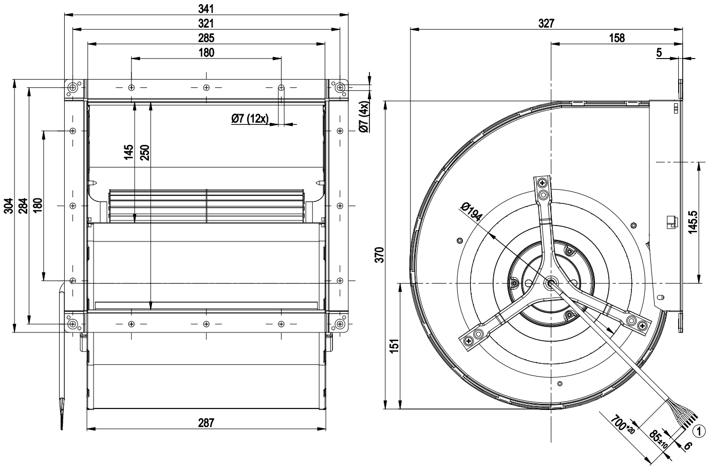
1 Connection line ETFE AWG20, 6x lead tips crimped
