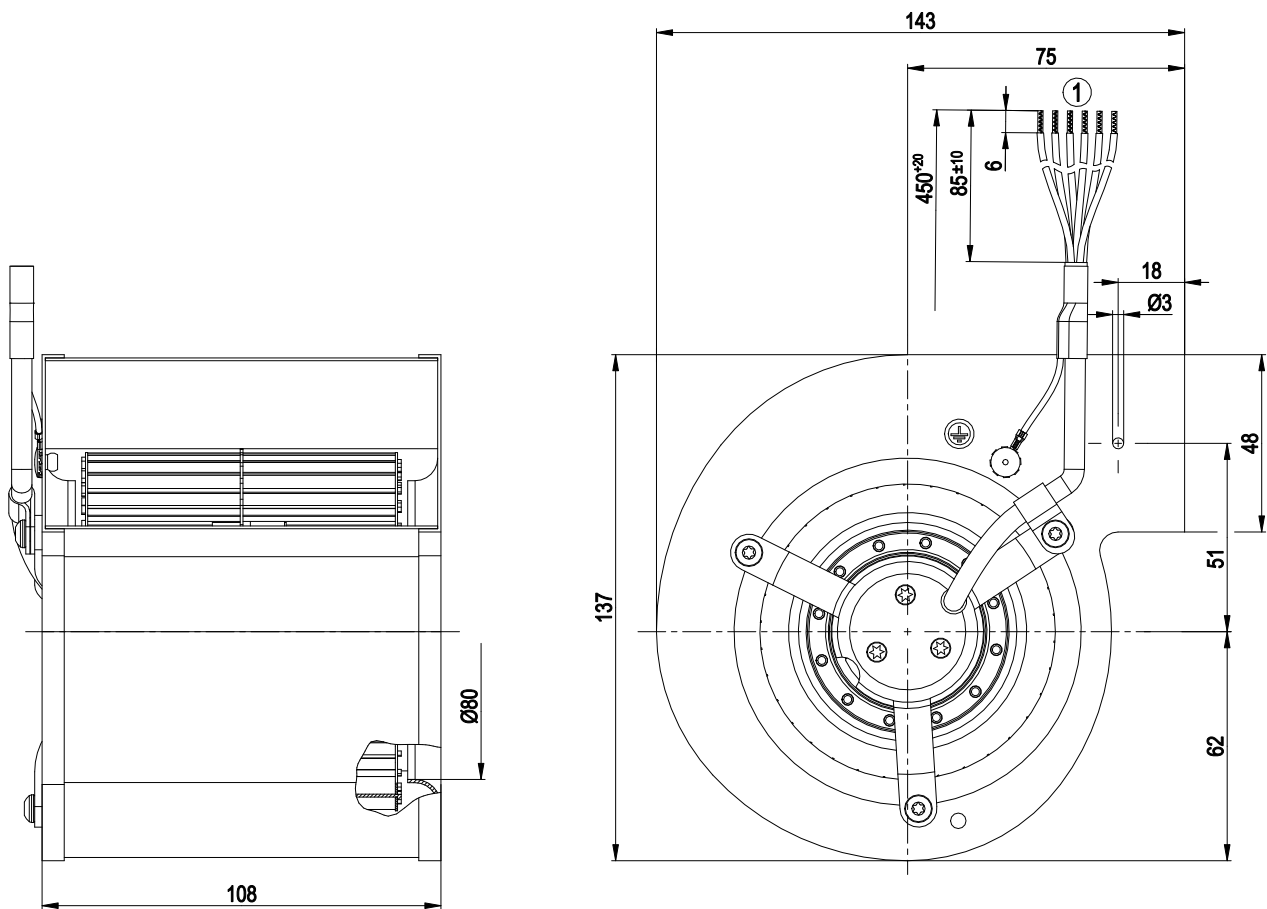
1 Cable PVC AWG22, 6x crimped splices
