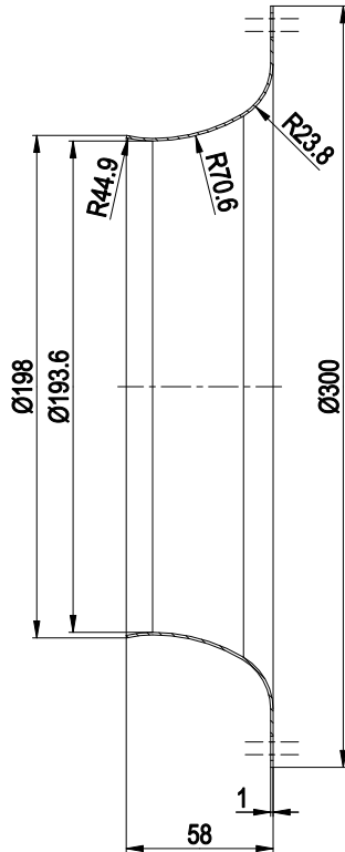
Inlet ring 31000-2-4013
