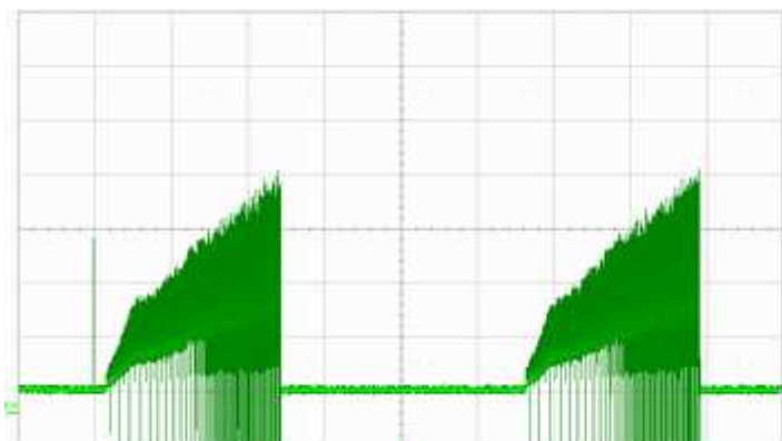
Locked rotor current at 48,0 V; I=500mA/Div, t=1s/Div
