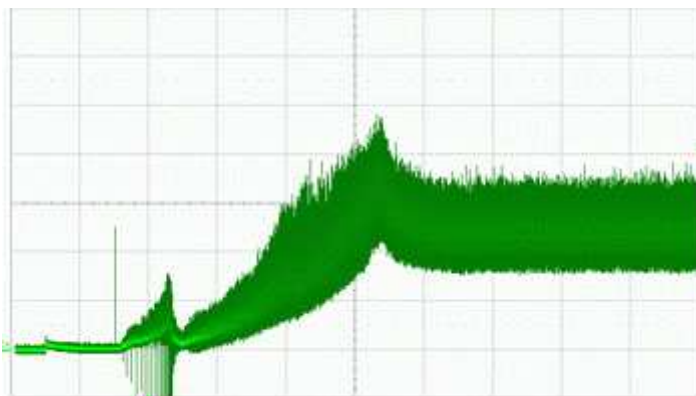
Start-up current at 48,0 V; I=500mA/Div, t=2s/Div
