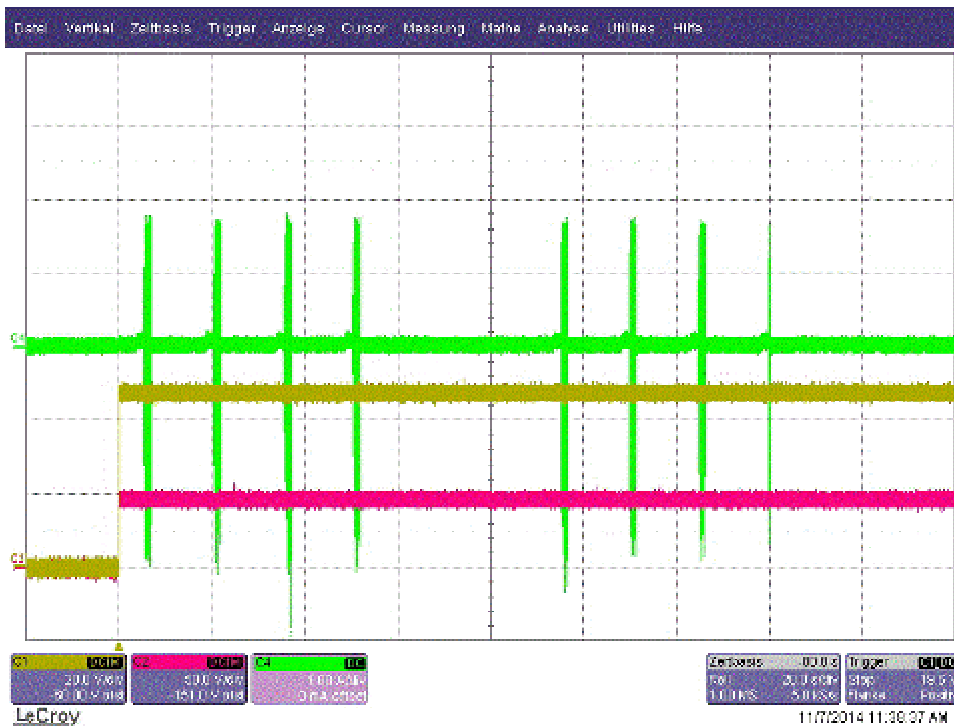
Start-up current @ 48 V ( I = 1\text{A/div} ; t = 2\text{s/div} )
