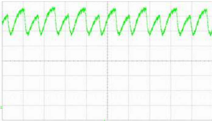
Running current @ 24 V (I = 1A/div ; t = 500us/div)
