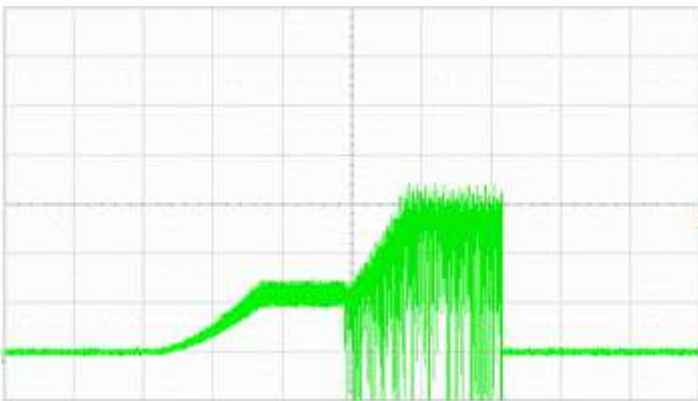
Locked rotor current @ 24 V (I = 2A/div ; t = 1s/div)
