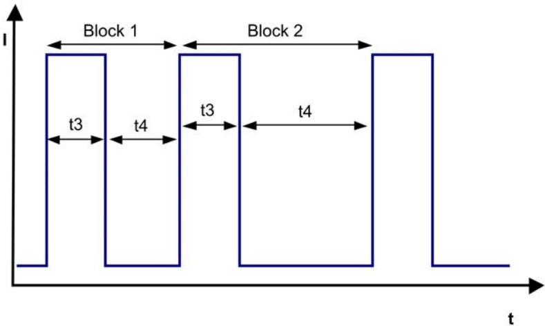
Block1: special locked rotor protection: 5 cycles t_3 / t_4 = 0,6\text{ s} / 1\text{ s} Block2: locked rotor protection t_3 / t_4 = 0,6\text{ s} / 10\text{ s}
