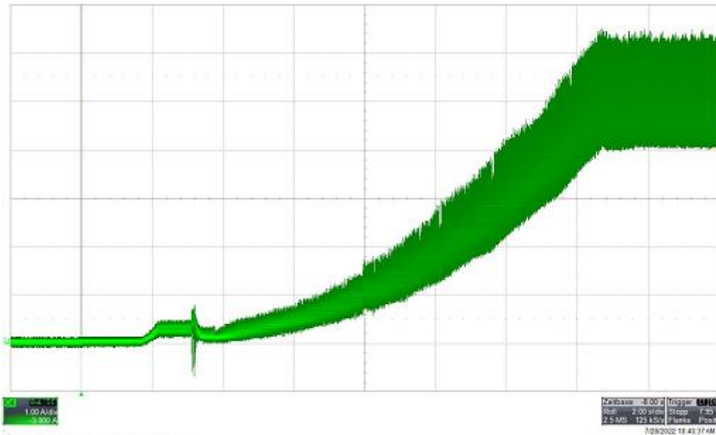
Startup current @ 24V, 0 - 11000 rpm
