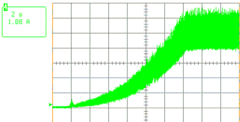
Startup current @ 24V, 0 - 11000 rpm
