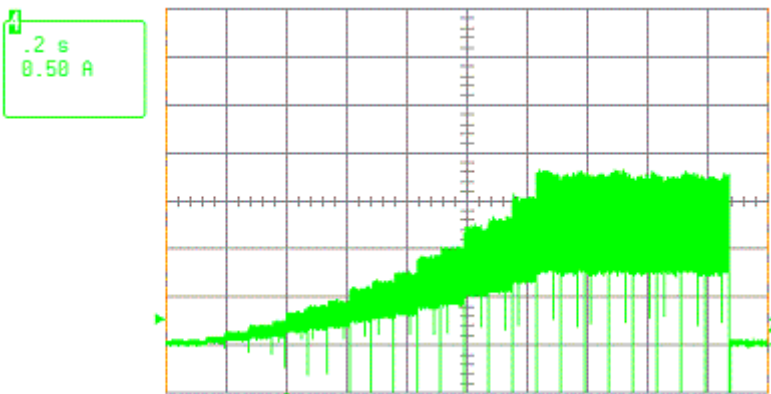
Locked rotor current @ 24V
