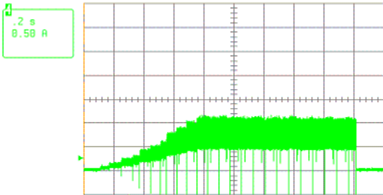
Locked rotor current @ 30V
