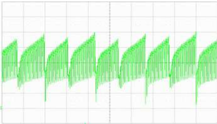
Running current @ 48 V ( I = 200\text{mA/div} ; t = 1\text{ms/div} )
