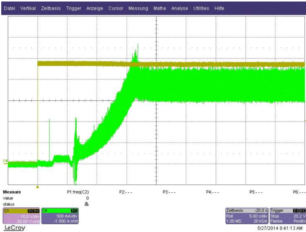
Start_up current @ 48V
