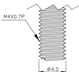
MECHANICAL SCREW
