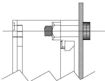
MOUNTING DRAWING
