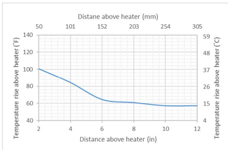
Temperature rise vs. distance above heater
