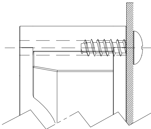
MOUNTING DRAWING
